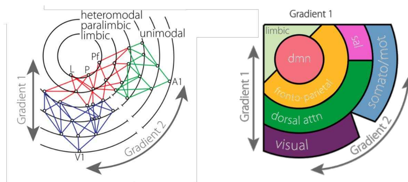
Fig. 5. The Mesulam model (left) and the Margulies model (right) of the cortical abstraction hierarchy. Adapted from Margulies et al. (2016).
